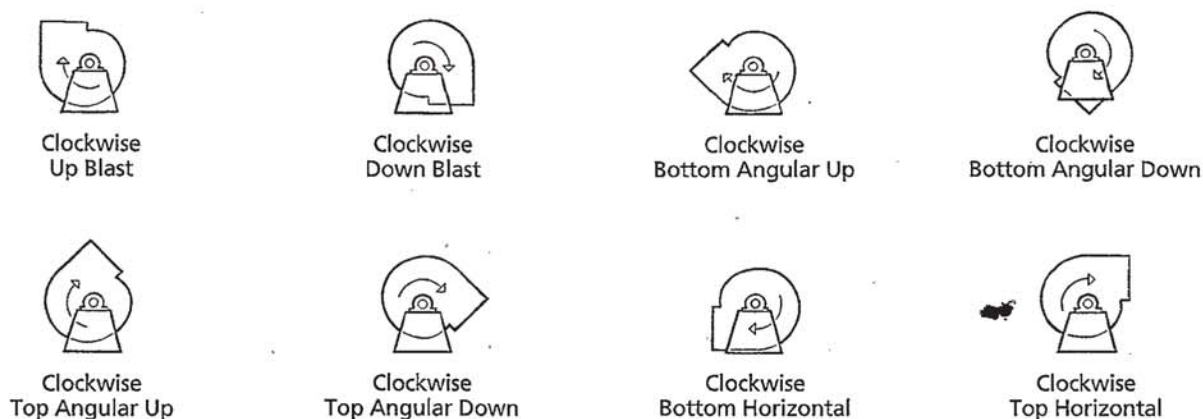
Figure 2 – Adjustable Blower Discharge Positions
